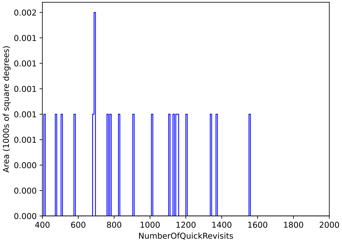
too_elab_r256_d2_gz_v3.4_10yrs : NumberOfQuickRevisits
