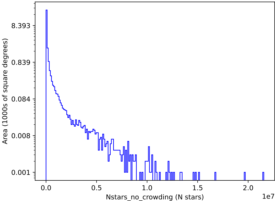
too_elab_r256_d2_gz_v3.4_10yrs r: Nstars_no_crowding
