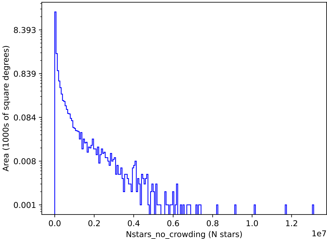
too_elab_r256_d2_gz_v3.4_10yrs g: Nstars_no_crowding
