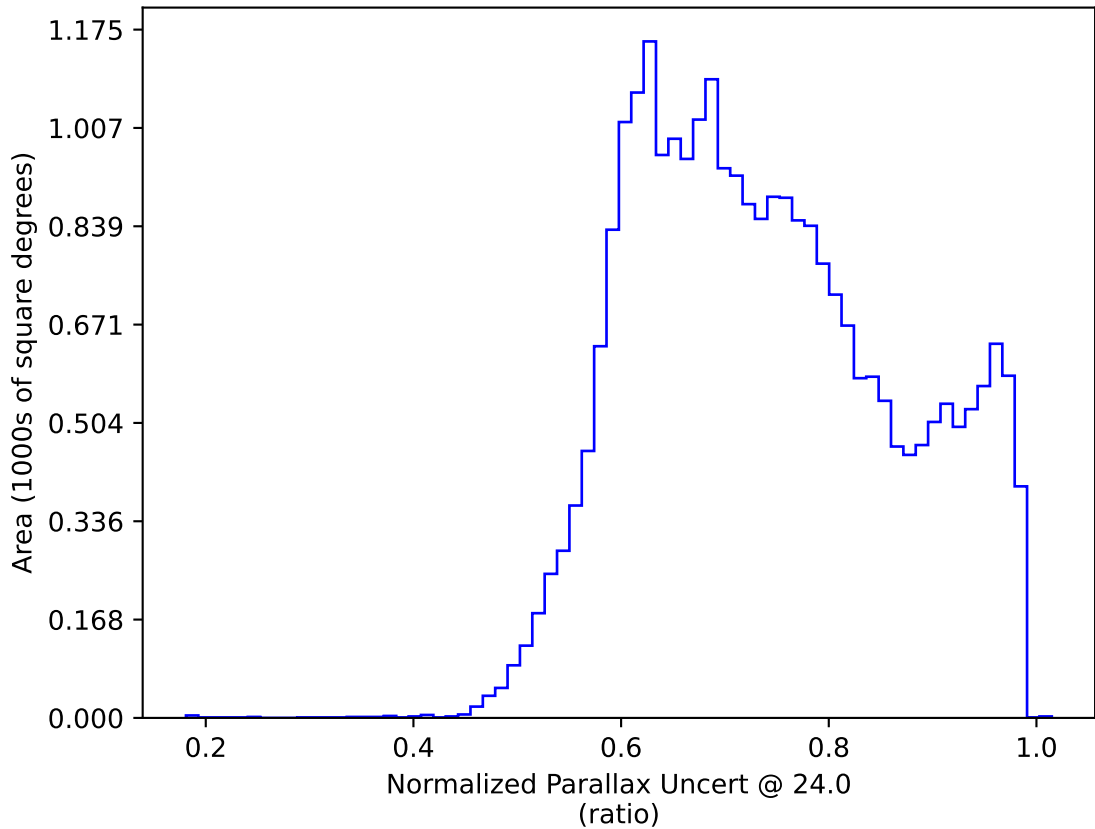
too_elab_r256_d2_gz_v3.4_10yrs : Normalized Parallax Uncert @ 24.0
