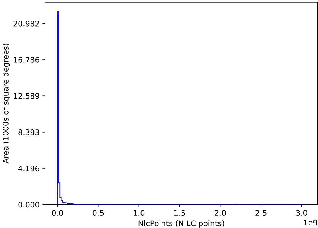
too_elab_r256_d2_gz_v3.4_10yrs : NlcPoints
