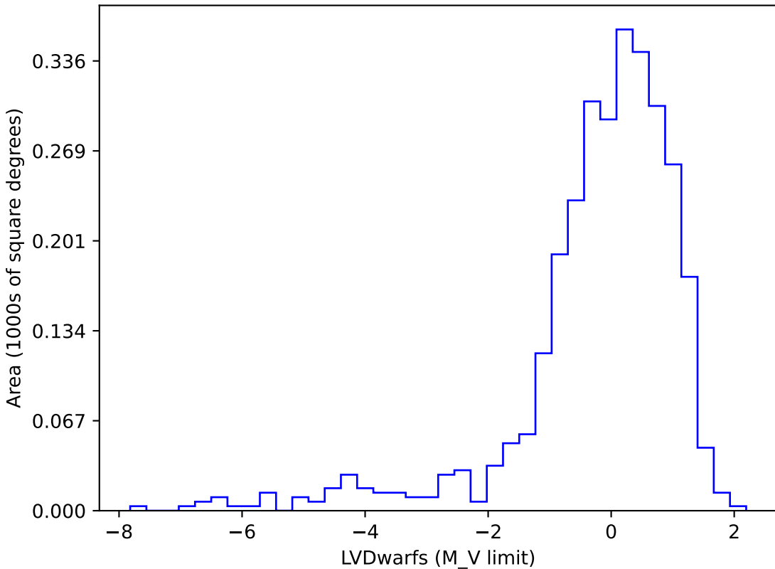
too_elab_r256_d2_gz_v3.4_10yrs gi SCP: LVDwarfs
