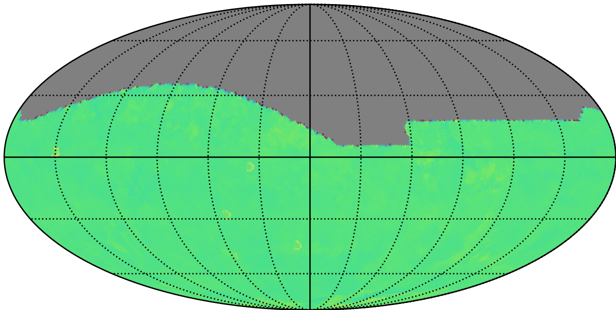
too_elab_r256_d2_gz_v3.4_10yrs r: Kuiper rotTelPos
