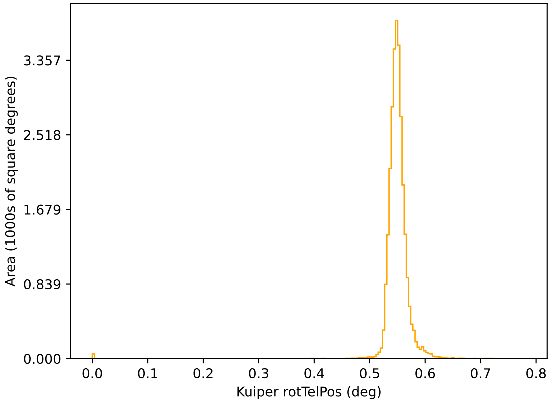
too_elab_r256_d2_gz_v3.4_10yrs r: Kuiper rotTelPos
