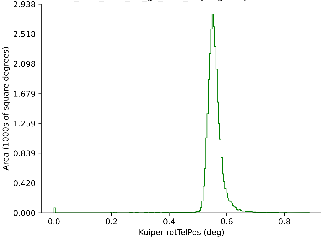
too_elab_r256_d2_gz_v3.4_10yrs g: Kuiper rotTelPos
