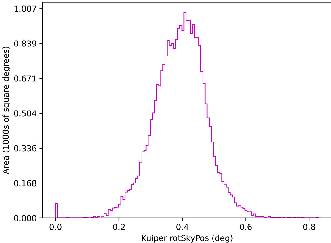
too_elab_r256_d2_gz_v3.4_10yrs z: Kuiper rotSkyPos
