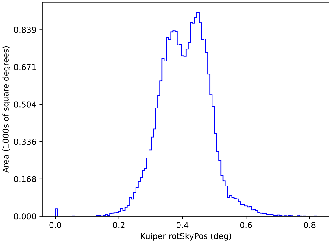
too_elab_r256_d2_gz_v3.4_10yrs y: Kuiper rotSkyPos
