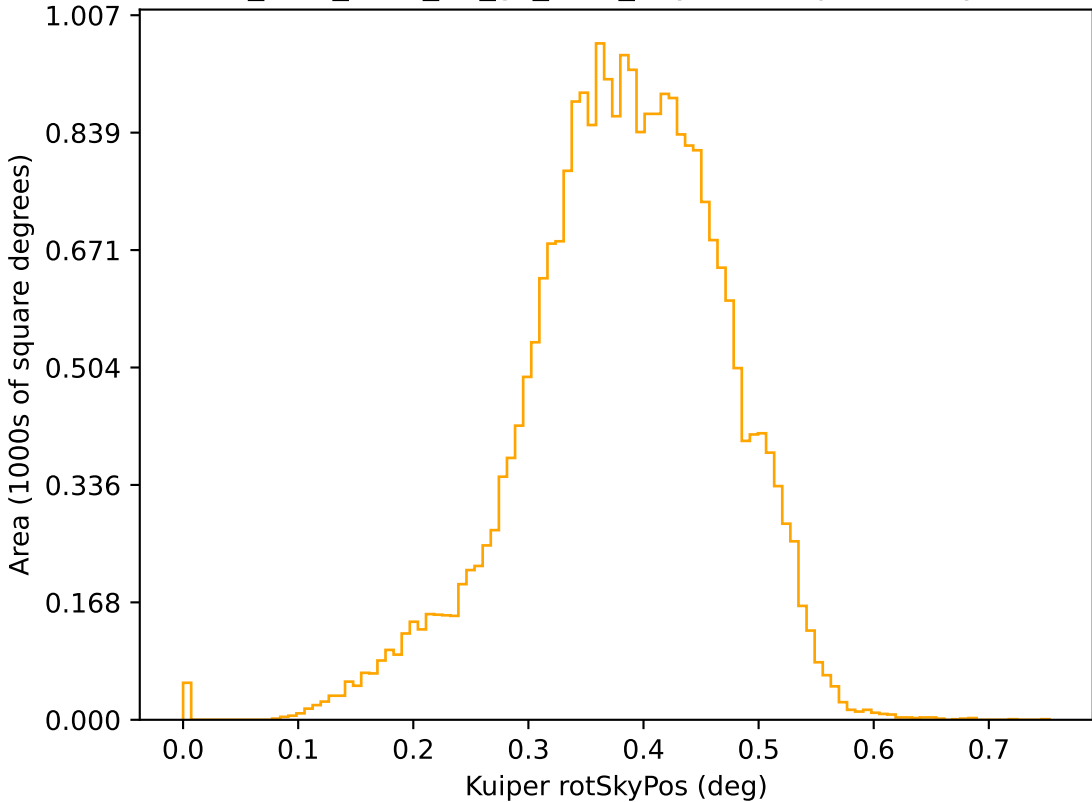
too_elab_r256_d2_gz_v3.4_10yrs r: Kuiper rotSkyPos
