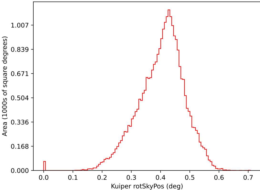
too_elab_r256_d2_gz_v3.4_10yrs i: Kuiper rotSkyPos
