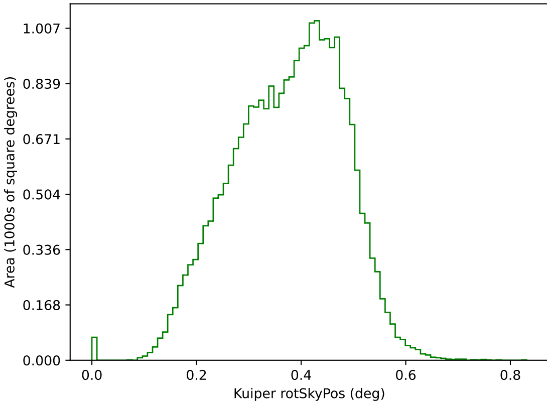
too_elab_r256_d2_gz_v3.4_10yrs g: Kuiper rotSkyPos
