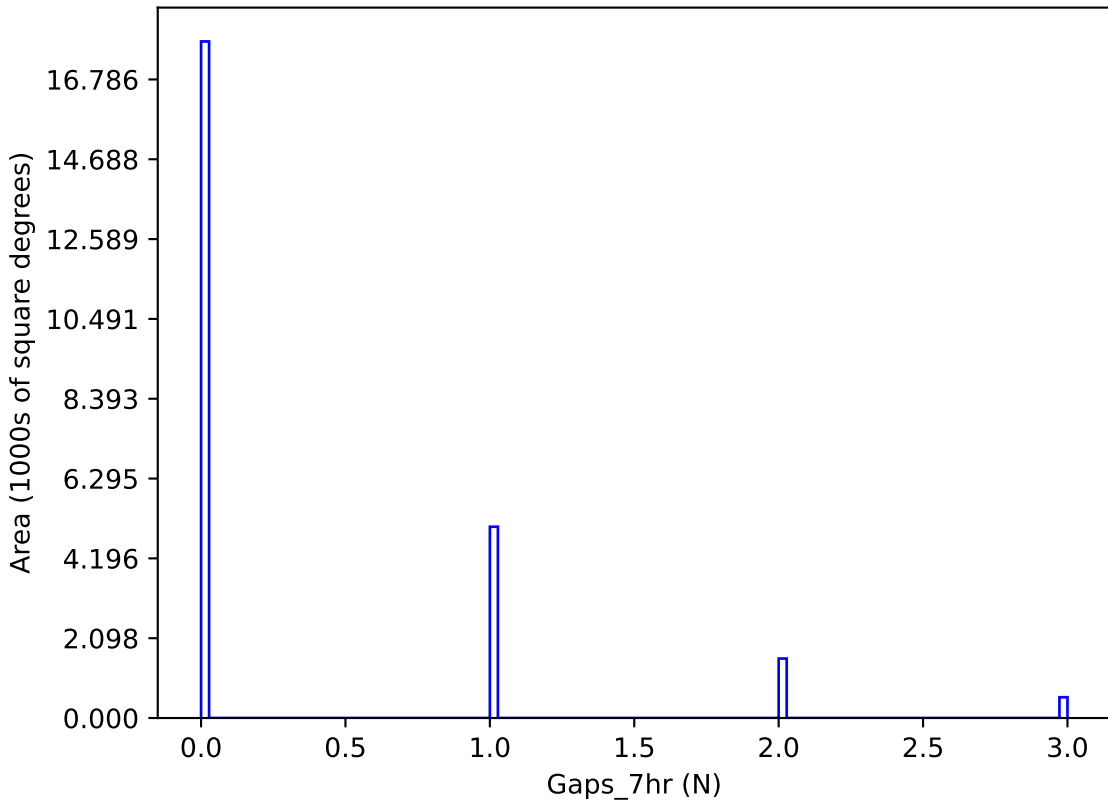
too_elab_r256_d2_gz_v3.4_10yrs y band: Gaps_7hr
