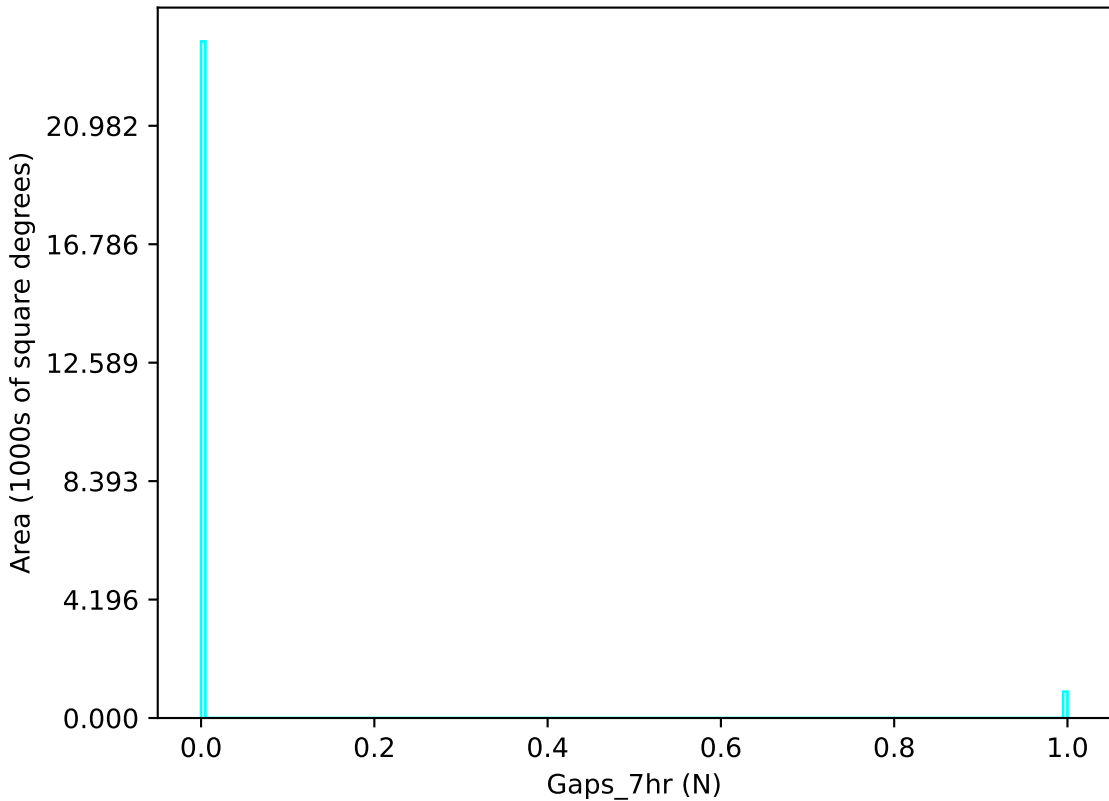
too_elab_r256_d2_gz_v3.4_10yrs u band: Gaps_7hr
