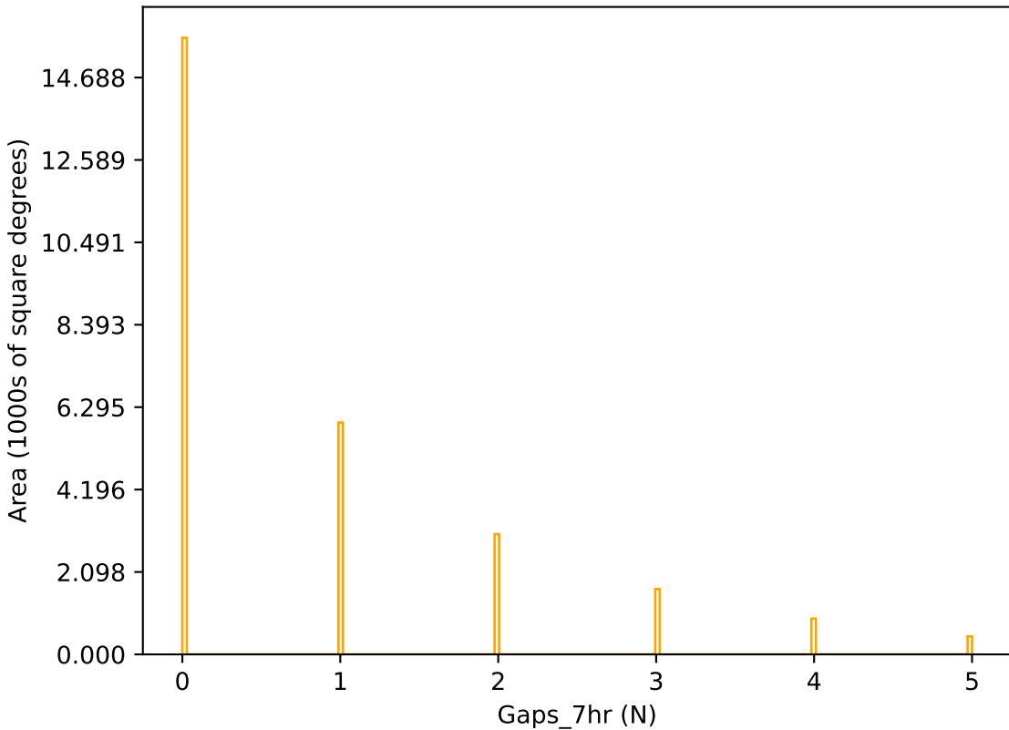
too_elab_r256_d2_gz_v3.4_10yrs r band: Gaps_7hr
