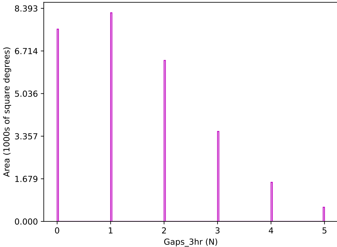
too_elab_r256_d2_gz_v3.4_10yrs z band: Gaps_3hr
