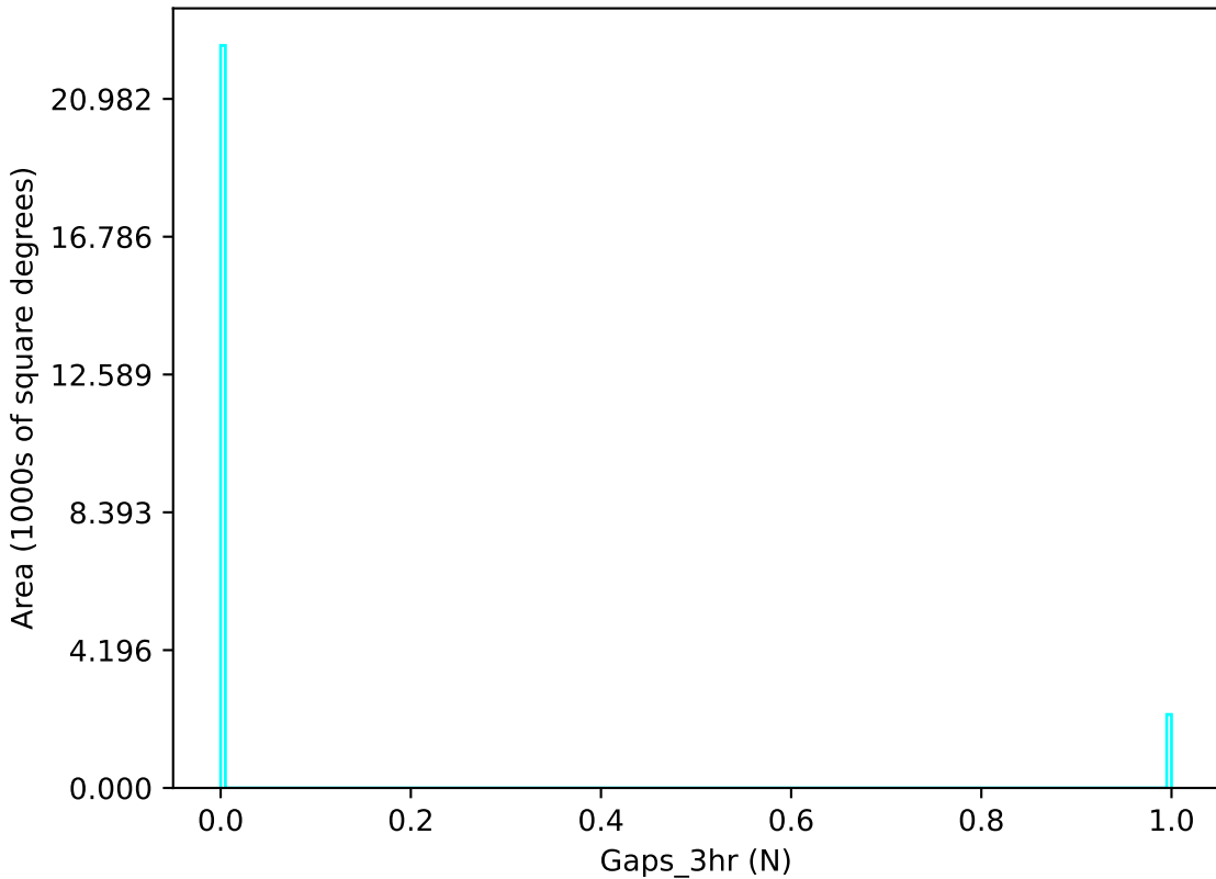
too_elab_r256_d2_gz_v3.4_10yrs u band: Gaps_3hr
