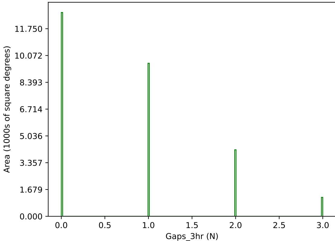
too_elab_r256_d2_gz_v3.4_10yrs g band: Gaps_3hr
