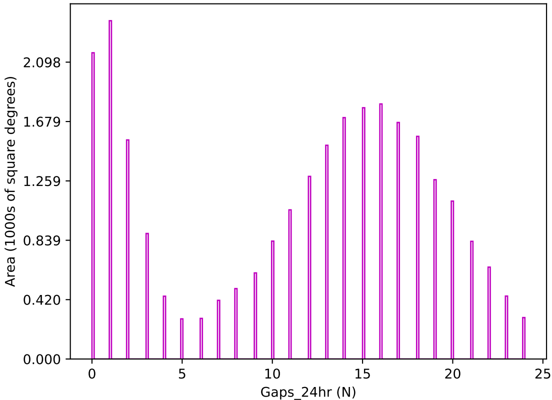
too_elab_r256_d2_gz_v3.4_10yrs z band: Gaps_24hr
