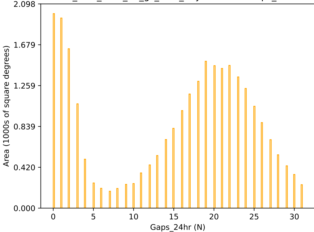
too_elab_r256_d2_gz_v3.4_10yrs r band: Gaps_24hr
