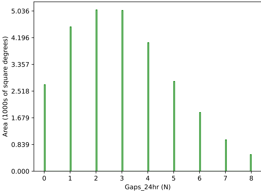
too_elab_r256_d2_gz_v3.4_10yrs g band: Gaps_24hr
