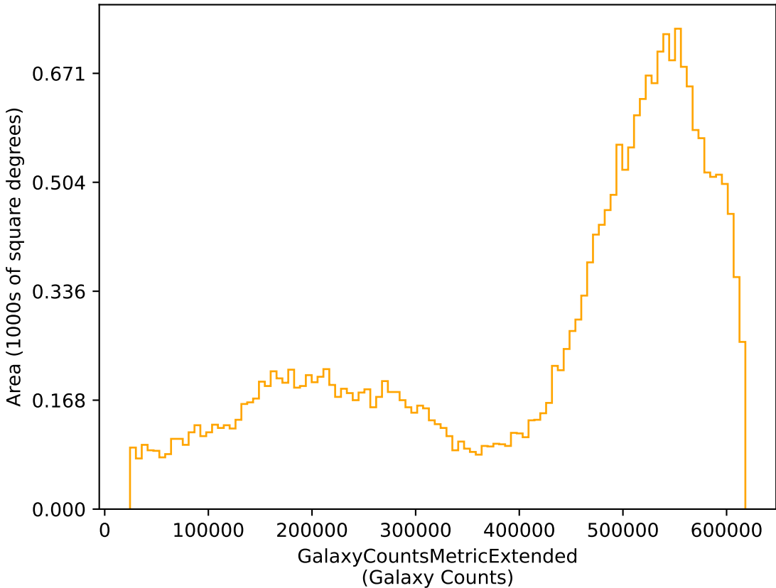
too_elab_r256_d2_gz_v3.4_10yrs r: GalaxyCountsMetricExtended
