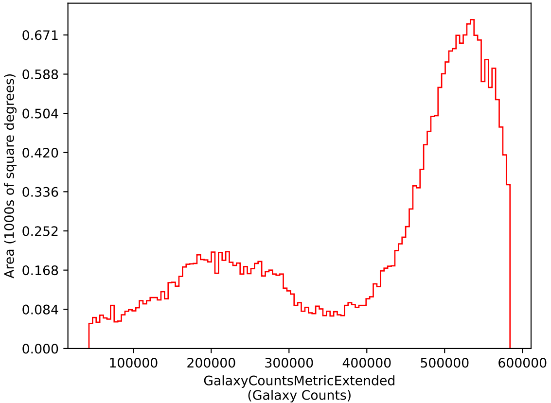
too_elab_r256_d2_gz_v3.4_10yrs i: GalaxyCountsMetricExtended
