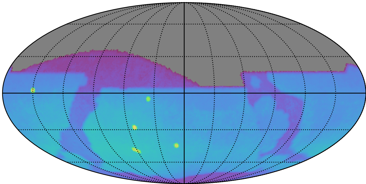
too_elab_r256_d2_gz_v3.4_10yrs : Brown Dwarf, L7
