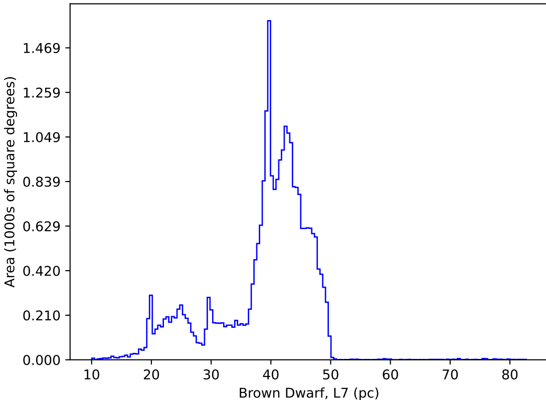
too_elab_r256_d2_gz_v3.4_10yrs : Brown Dwarf, L7
