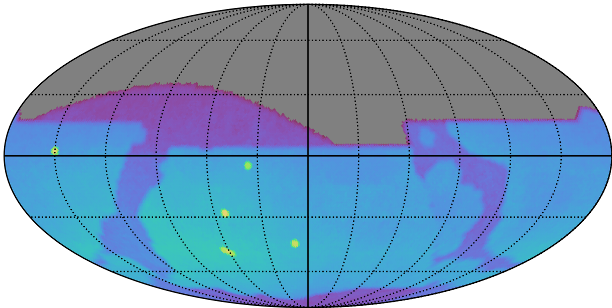
too_elab_r256_d2_gz_v3.4_10yrs : Brown Dwarf, L4
