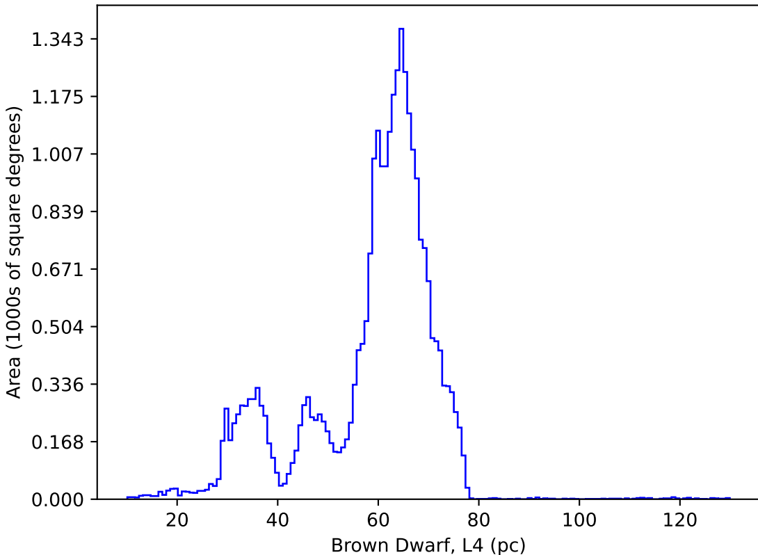
too_elab_r256_d2_gz_v3.4_10yrs : Brown Dwarf, L4
