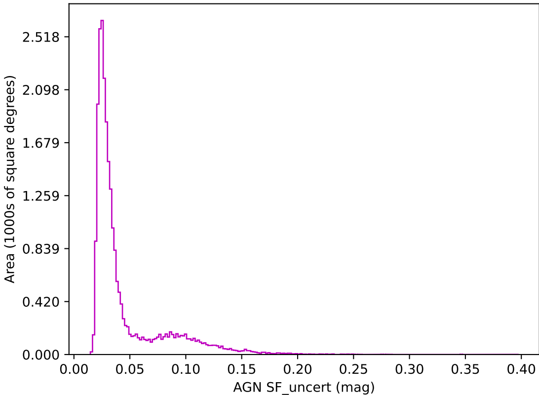
too_elab_r256_d2_gz_v3.4_10yrs z band: AGN SF_uncert
