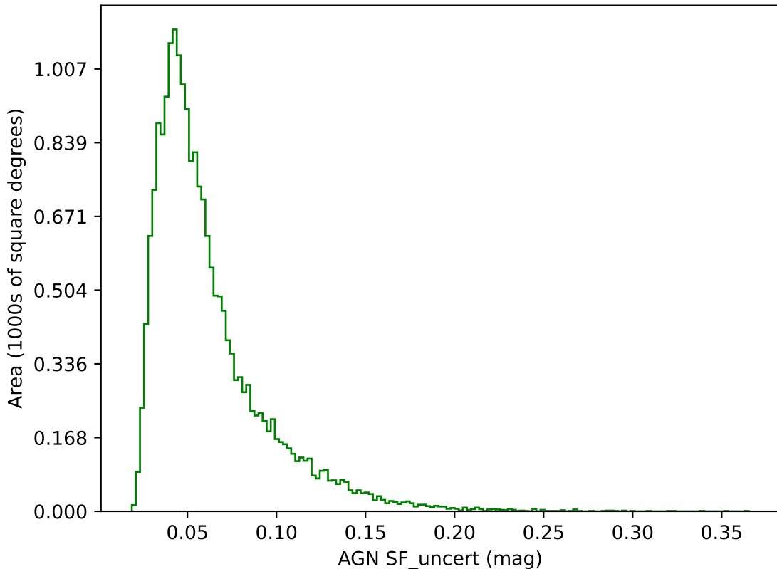
too_elab_r256_d2_gz_v3.4_10yrs g band: AGN SF_uncert
