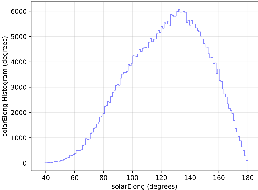
too_elab_r256_d2_gz_v3.4_10yrs WFD y band: solarElong Histogram
