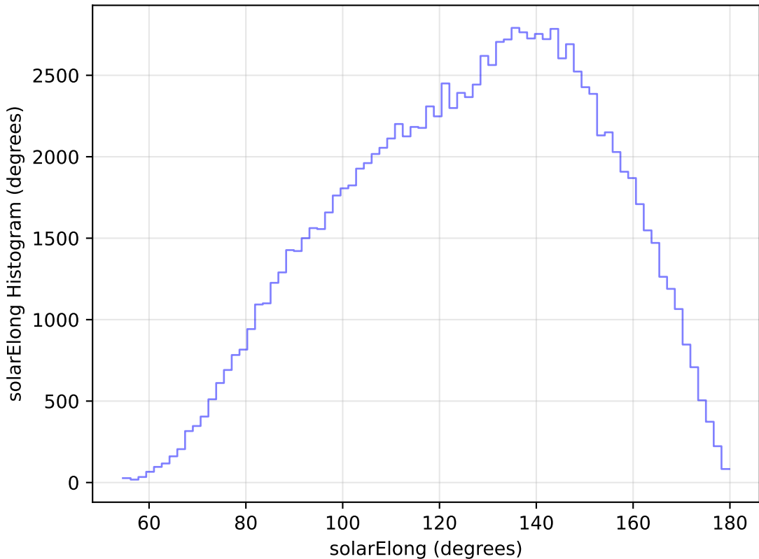
too_elab_r256_d2_gz_v3.4_10yrs WFD u band: solarElong Histogram
