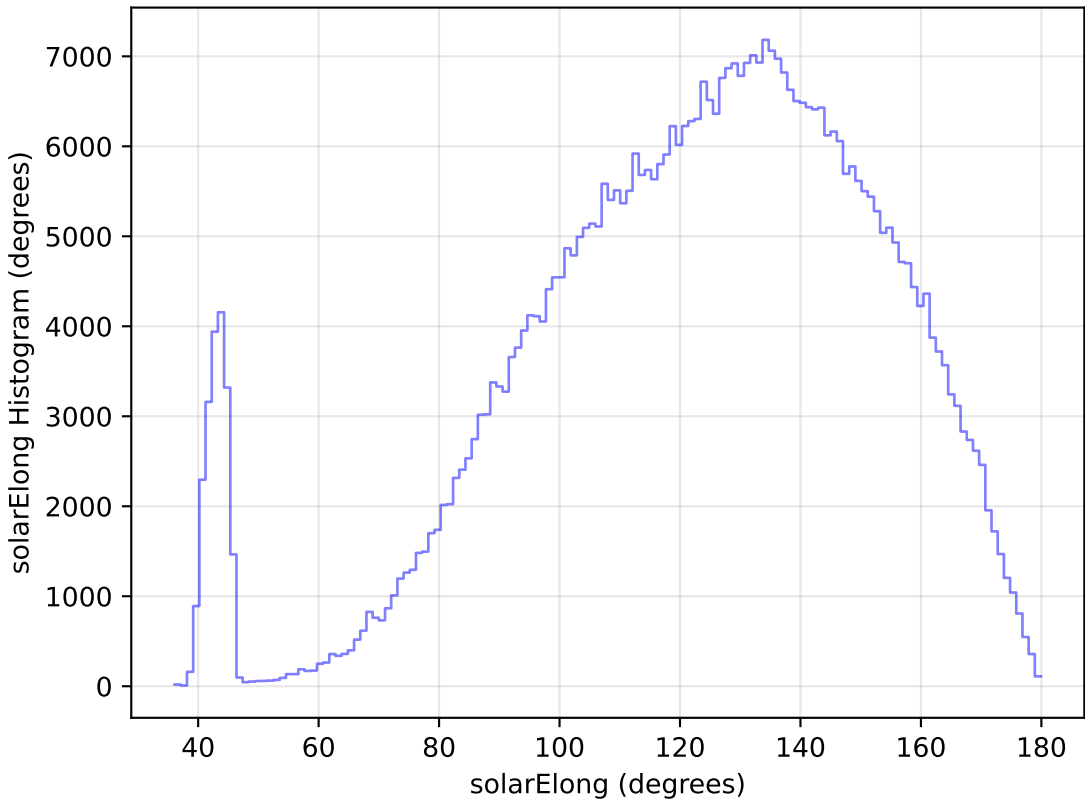
too_elab_r256_d2_gz_v3.4_10yrs WFD r band: solarElong Histogram
