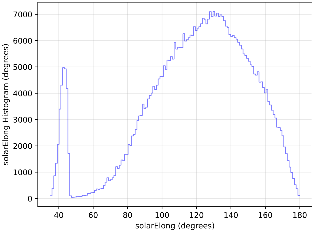
too_elab_r256_d2_gz_v3.4_10yrs WFD i band: solarElong Histogram
