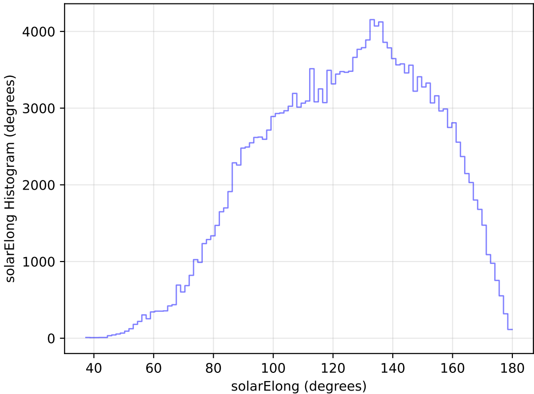
too_elab_r256_d2_gz_v3.4_10yrs WFD g band: solarElong Histogram
