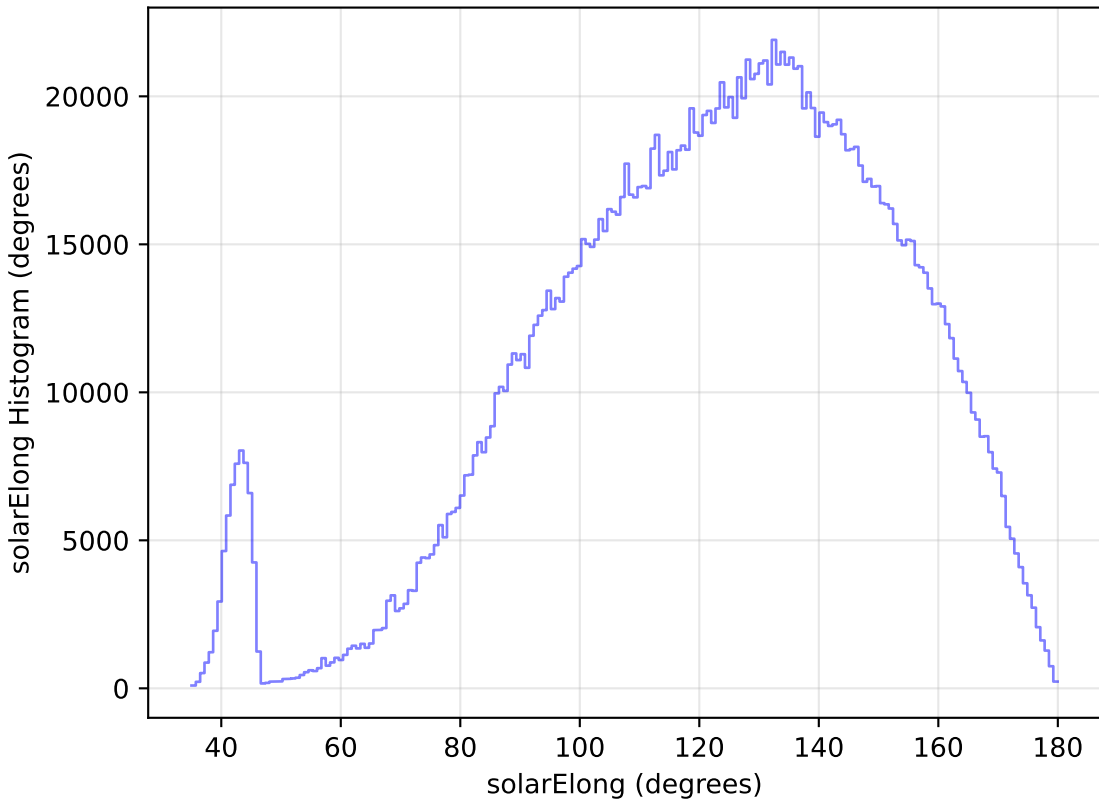
too_elab_r256_d2_gz_v3.4_10yrs WFD all bands: solarElong Histogram
