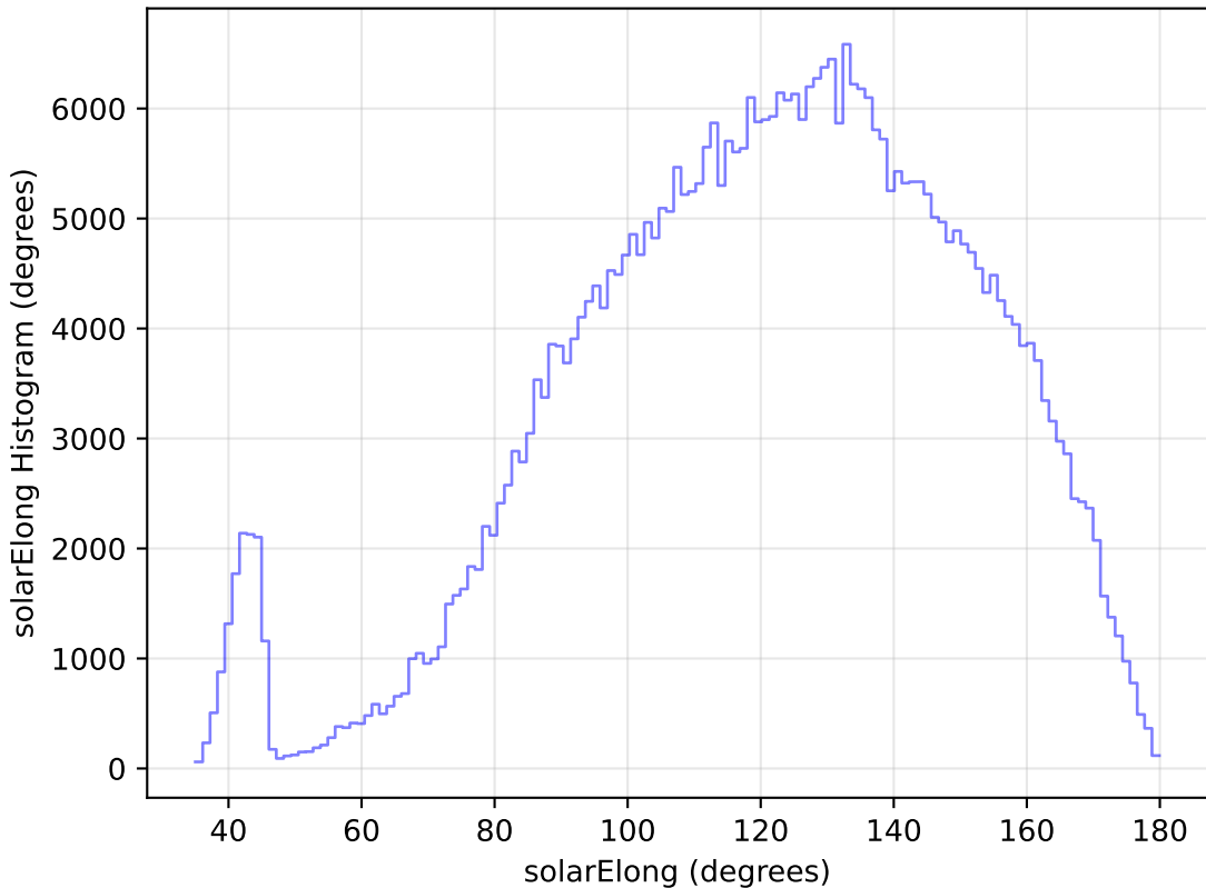
too_elab_r256_d2_gz_v3.4_10yrs All sky z band: solarElong Histogram
