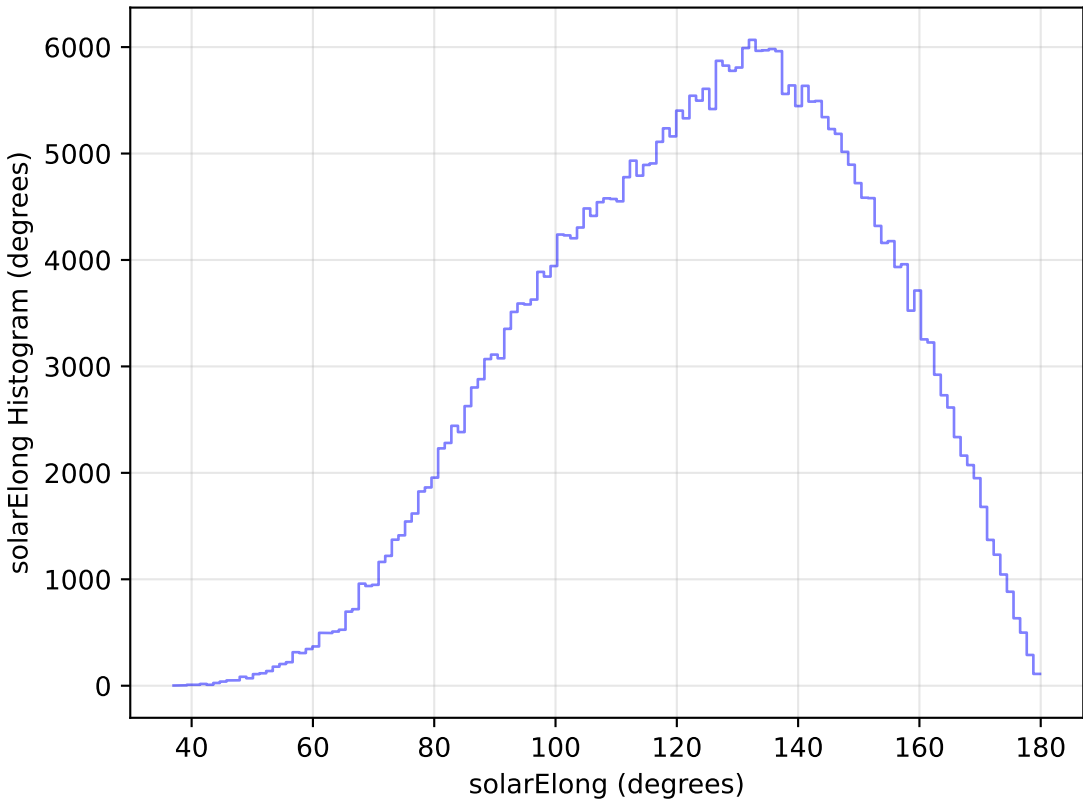
too_elab_r256_d2_gz_v3.4_10yrs All sky y band: solarElong Histogram
