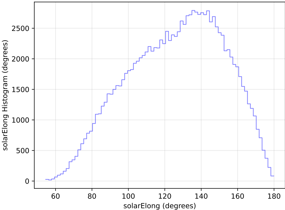
too_elab_r256_d2_gz_v3.4_10yrs All sky u band: solarElong Histogram
