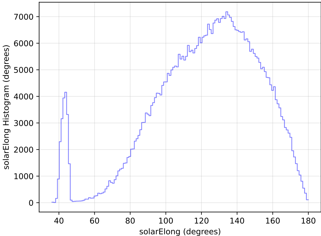
too_elab_r256_d2_gz_v3.4_10yrs All sky r band: solarElong Histogram
