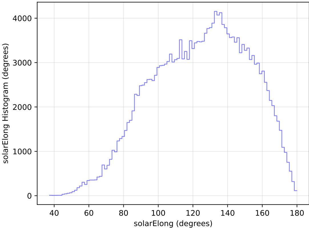
too_elab_r256_d2_gz_v3.4_10yrs All sky g band: solarElong Histogram
