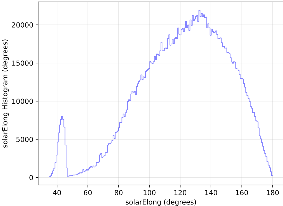
too_elab_r256_d2_gz_v3.4_10yrs All sky all bands: solarElong Histogram
