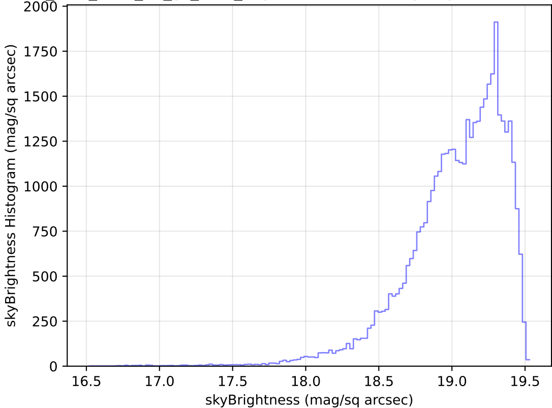
too_elab_r256_d2_gz_v3.4_10yrs Yr 1 z band: skyBrightness Histogram
