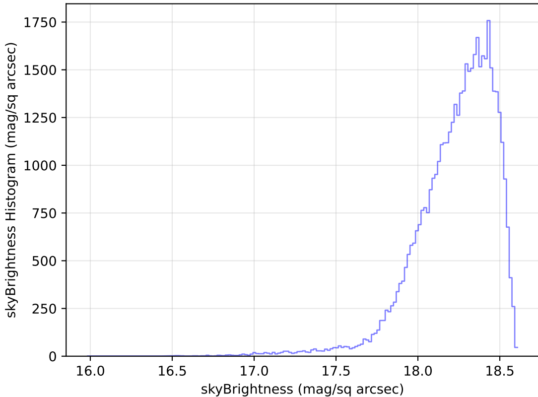
too_elab_r256_d2_gz_v3.4_10yrs Yr 1 y band: skyBrightness Histogram
