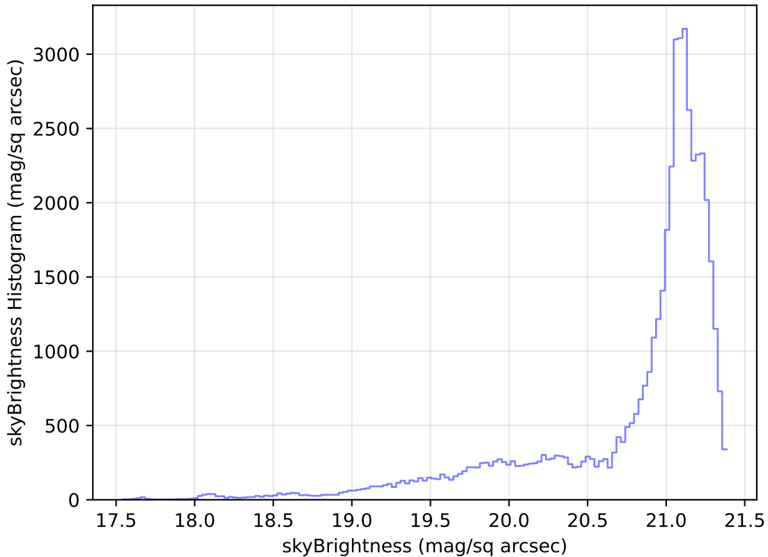
too_elab_r256_d2_gz_v3.4_10yrs Yr 1 r band: skyBrightness Histogram
