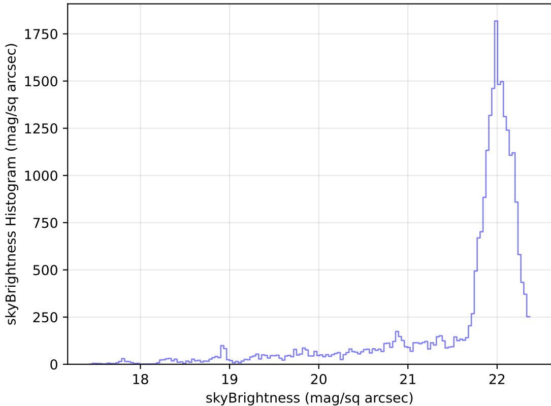
too_elab_r256_d2_gz_v3.4_10yrs Yr 1 g band: skyBrightness Histogram
