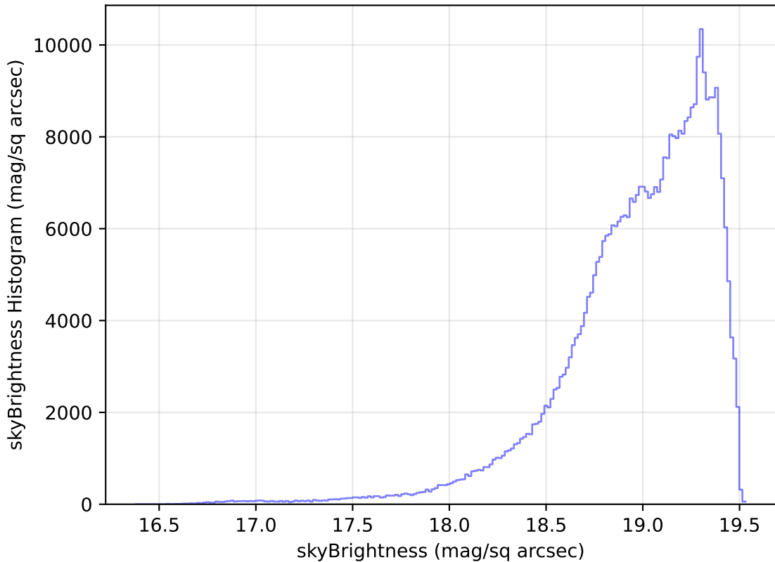
too_elab_r256_d2_gz_v3.4_10yrs WFD z band: skyBrightness Histogram
