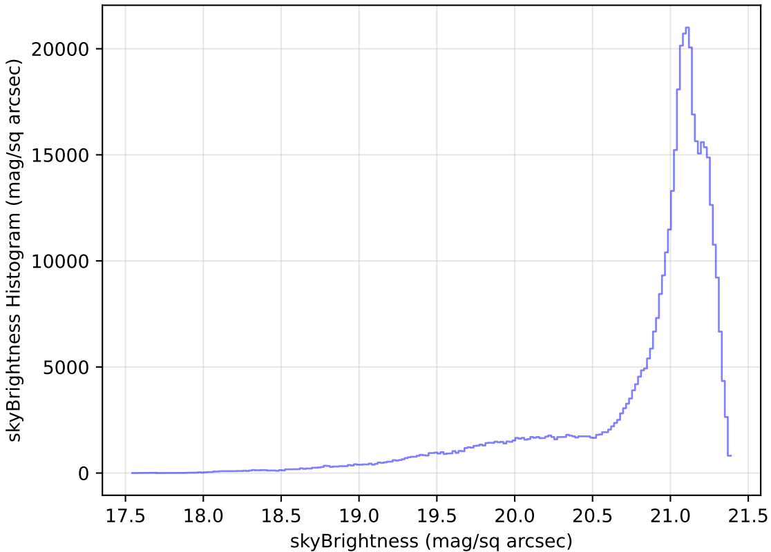
too_elab_r256_d2_gz_v3.4_10yrs WFD r band: skyBrightness Histogram
