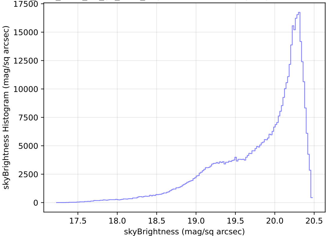
too_elab_r256_d2_gz_v3.4_10yrs WFD i band: skyBrightness Histogram
